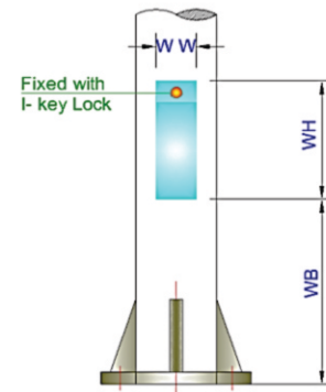
WINDOW DETAILS
