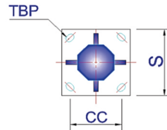
BASE PLATE DETAILS
