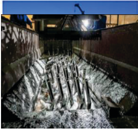
Hot Dip Galvanizing
